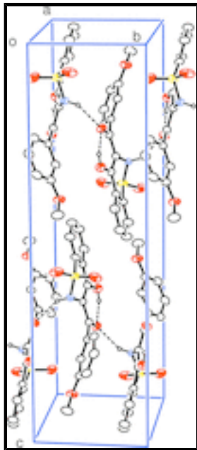
Fig. 2. A unit cell showing molecular packing of the title compound; hydrogen bonds are represented by dashed lines. The H-atoms not involved in H-bonds have been excluded for clarity.
