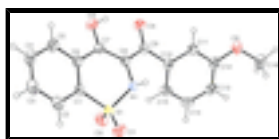
Fig. 1. The title molecule with the displacement ellipsoids plotted at 30% probability level (Farrugia, 1997).
